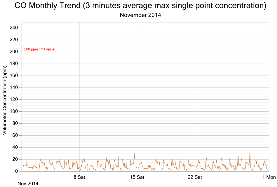
Figure 2: CO exposure and single point 3 minutes rolling averages for November 2014
