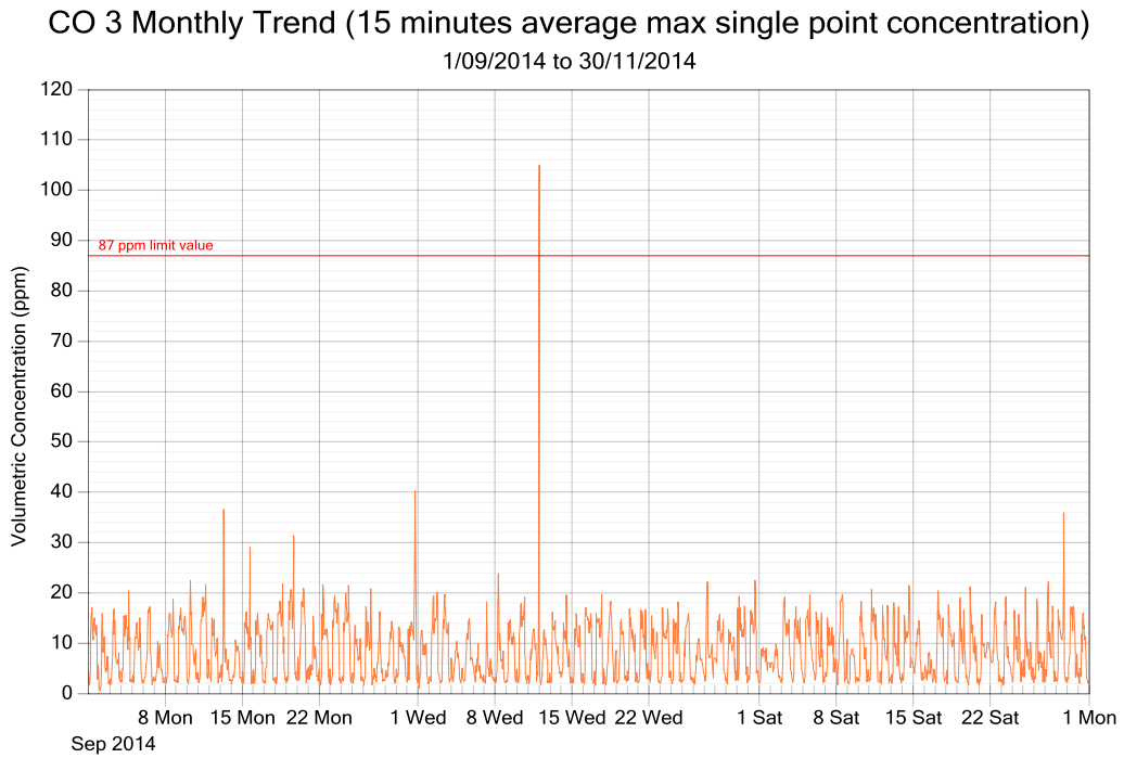
Figure 6: CO exposure and single point 15 minutes rolling averages from September to November 2014 (3 monthly trend)
