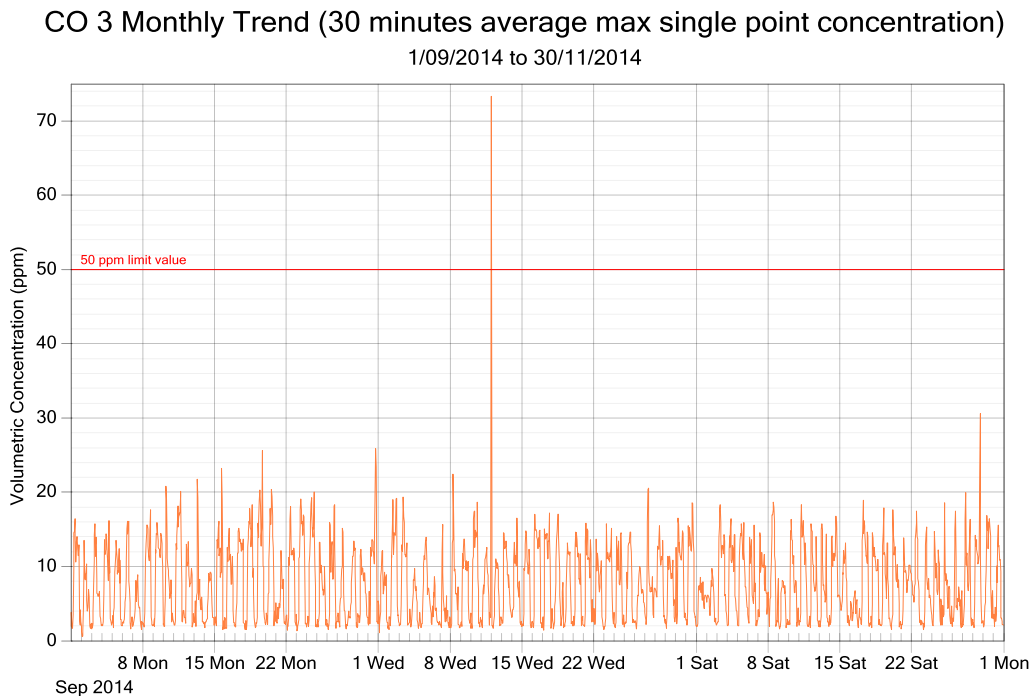
Figure 7: CO exposure and single point 30 minutes rolling averages from September to November 2014 (3 monthly trend)
