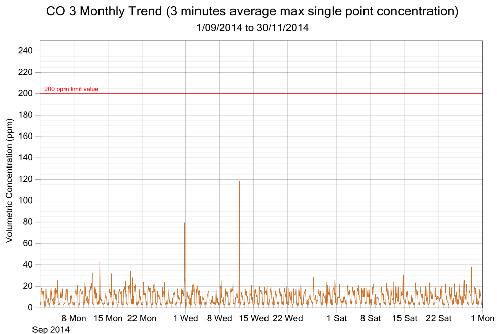
Figure 5: CO exposure and single point 3 minutes rolling averages from September to November 2014 (3 monthly trend)
