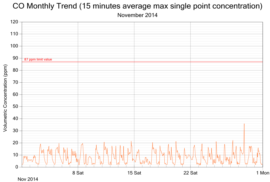
Figure 3: CO exposure and single point 15 minutes rolling averages for November 2014
