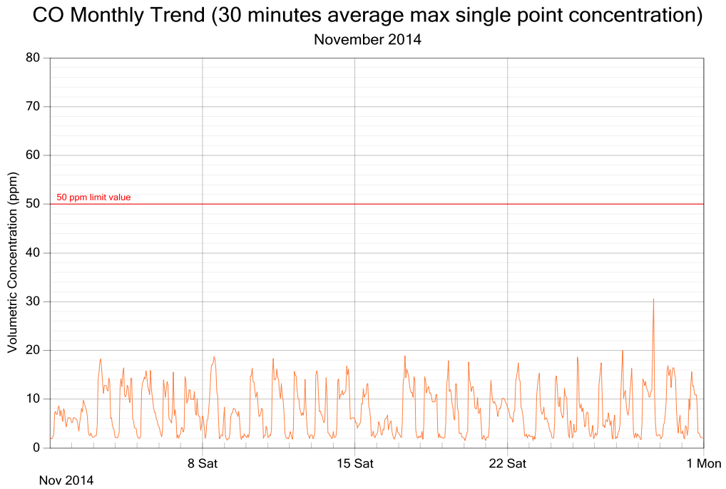
Figure 4: CO exposure and single point 30 minutes rolling averages for November 2014
